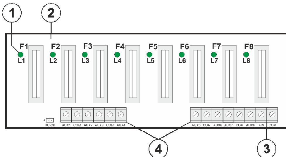
Fig.2. The view of the PSU's PCB.
