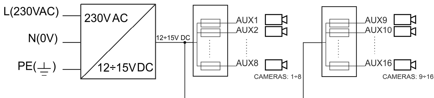
Fig.1. Block diagram of the PSU.
