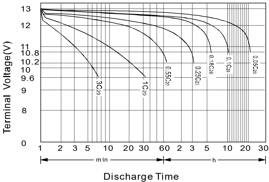
Discharge Characteristics Curve (25°C, 68°F)
