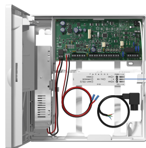
MG5075 with 110-220V / 75W Internal Power Supply
