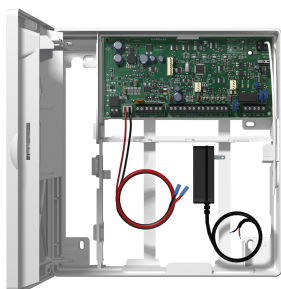
MG5075 with 110-220V / 15 Vdc / 60W Wall Plug
